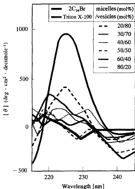
Fig. 3 CD Spectra of Z-PheHisLeu with 2C_{14}Br vesicles, coaggregates containing 20, 30, 40, 50, 60, 80, and 100 mol% Triton X-100 micelles ( \mu = 0.02 ).
