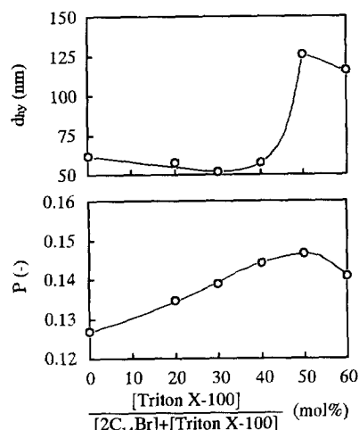
Fig. 2 Composition dependences of apparent hydrodynamic diameter ( d_{hy} ) and fluorescence polarization (P) of DPH in the Triton X-100 / 2C 14 Br coaggregates at 25°C and \mu = 0.02 .
