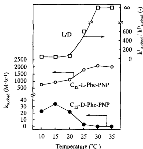
Fig. 4 Temperature dependence of rate constants ( k_{a,obsd} ) and enantioselectivity ( k_{a,obsd}^L / k_{a,obsd}^D ) for the hydrolysis of C_{12} -D(L)-Phe-PNP catalyzed by Z-PheHisLeu in the 30mol% Triton X-100 / 70mol% 2C_{14}Br coaggregates at pH 7.6 and \mu = 0.02 .
