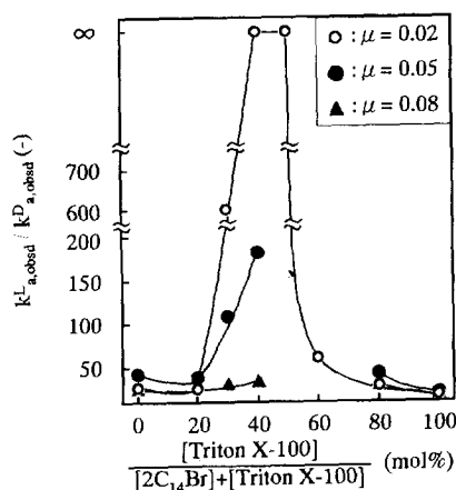
Fig. 1 Composition and ionic strength ( \mu ) dependences of enantioselectivity ( k_{a,obsd}^L / k_{a,obsd}^D ) for the hydrolysis of C 12 -D(L)-Phe-PNP catalyzed by Z-PheHisLeu in the Triton X-100 / 2C 14 Br coaggregates at 25°C and pH 7.6. [C 12 -D(L)-Phe-PNP] = 1.0 \times 10^{-5} M, [Z-PheHisLeu] = 5.0 \times 10^{-5} M.
